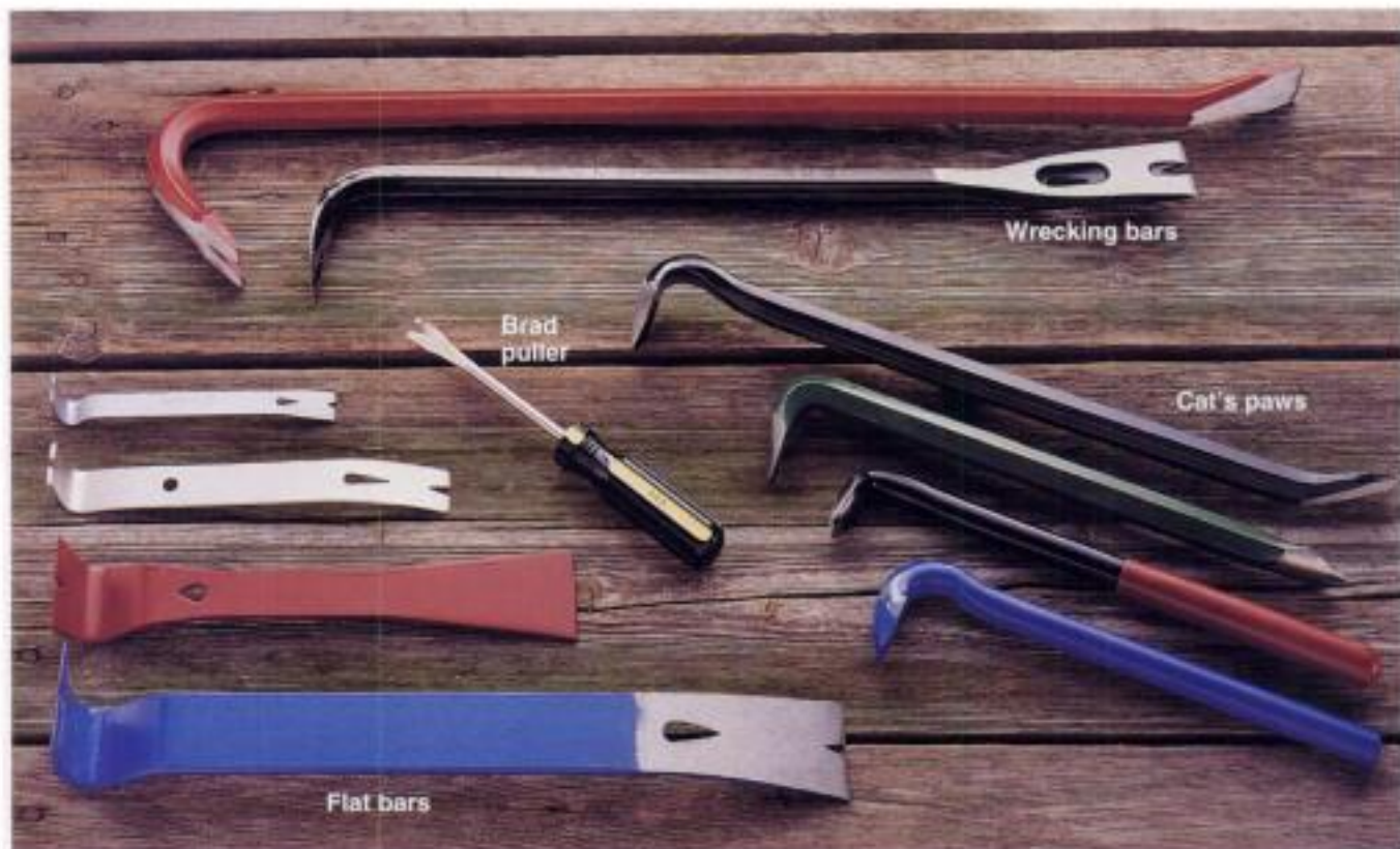
Prying tools include wrecking bars for heavy demolition work, cat's paws for removing nails, and a brad puller. Flat bars are made of flattened steel and come in a variety of sizes for light- and heavy-duty use.
